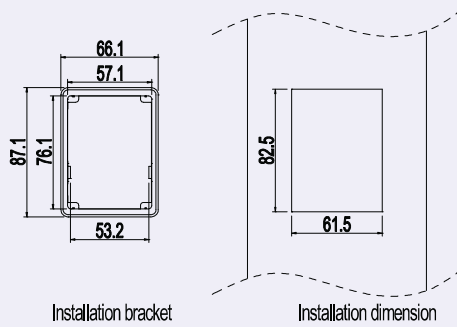
Installation bracket
