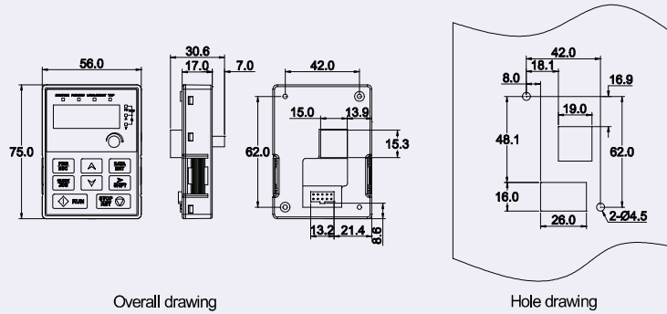
Overall drawing
